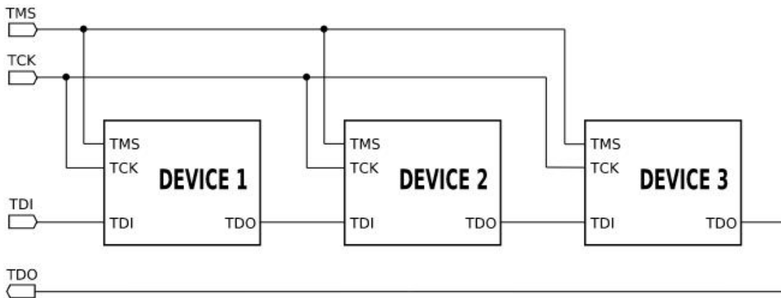
Figure 2.10.1a- Parallel Device JTAG Connection [A3]
