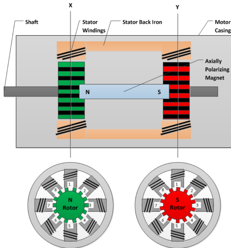
Figure 2.1.3a: Depiction of the Hybrid Stepper Motor construction
