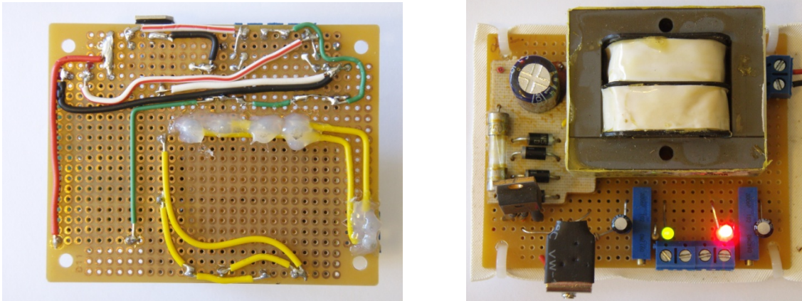
Figure 3.4c- Dual Voltage Power Supply (3.3v and 5v)
