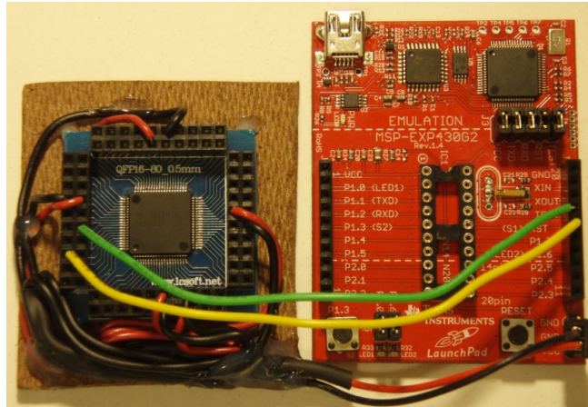
Figure 3.1d- Spy-Bi-Wire
