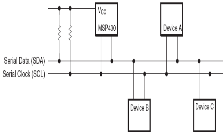
Figure 2.5.2b I 2 C Communication [L-8]
