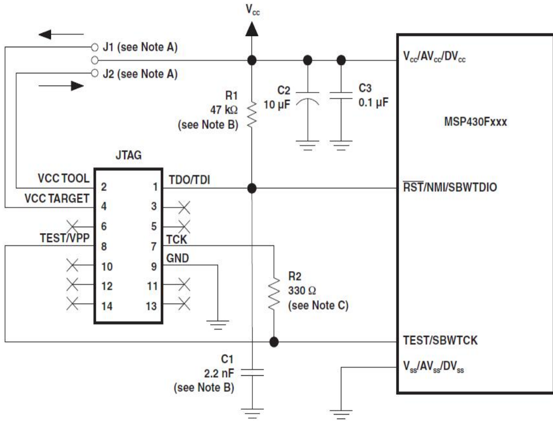
Figure 4.6.8b- Recommended Spy-Bi-Wire Connection. [A4] This image is the recommended connection for Spy-Bi-Wire for the MSP430 line of microcontrollers. (Permission given by Texas Instruments)
