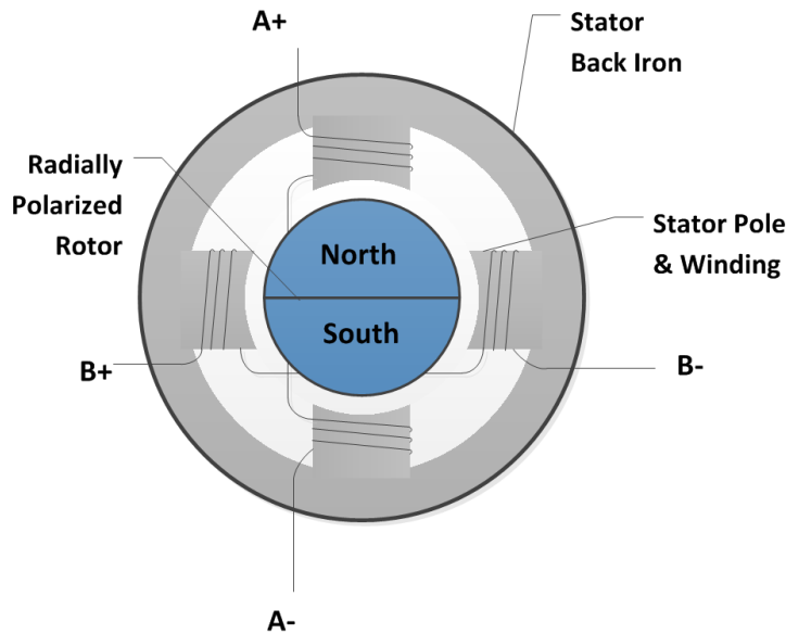
Figure 2.1b: Depiction of the permanent magnet stepper motor configuration
