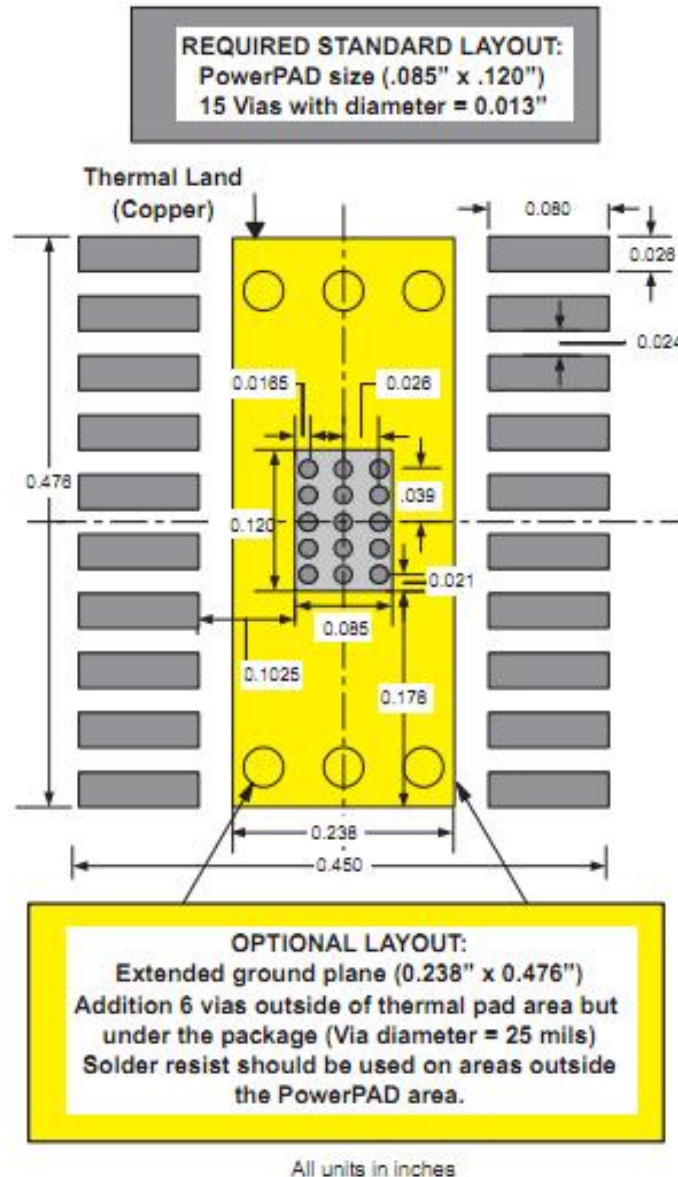
Figure 4.9.1a- PCB Layout for DRV8412 [A1] The required standard PCB layout for a PowerPad™ device. As shown, there are multiple vias required under the device. (Permission Granted by Texas Instruments)
