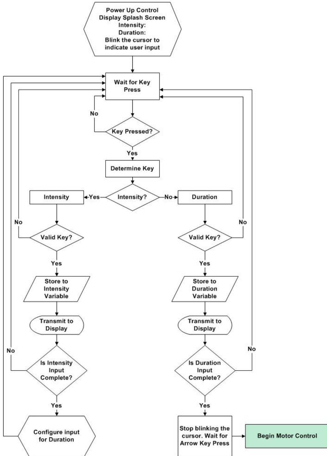
Figure 4.6.2a- User Interface Software Flowchart
