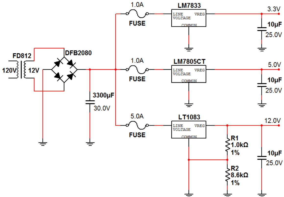
Figure 4.3.5b: Circuit Diagram for the Low Voltage Power Supply
