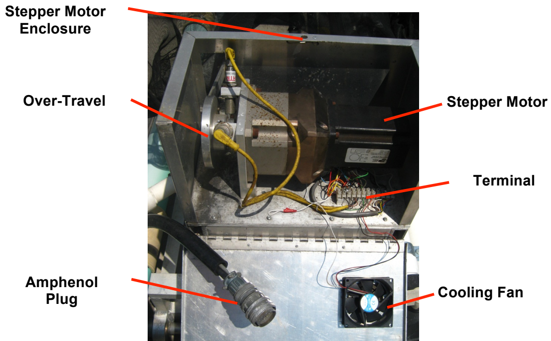
Figure 2.8a: Transmission Line End Items
