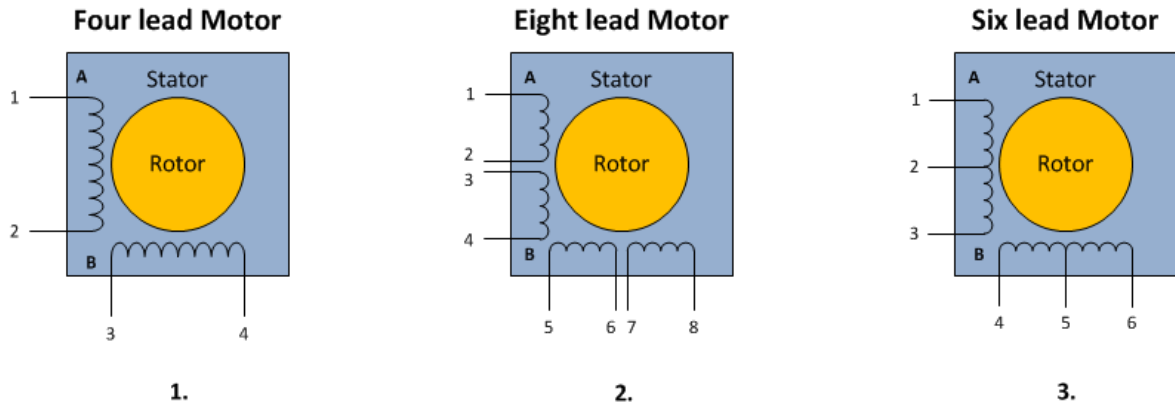
Figure 2.1.4a: Illustration of various options for stepper motor winding configurations
