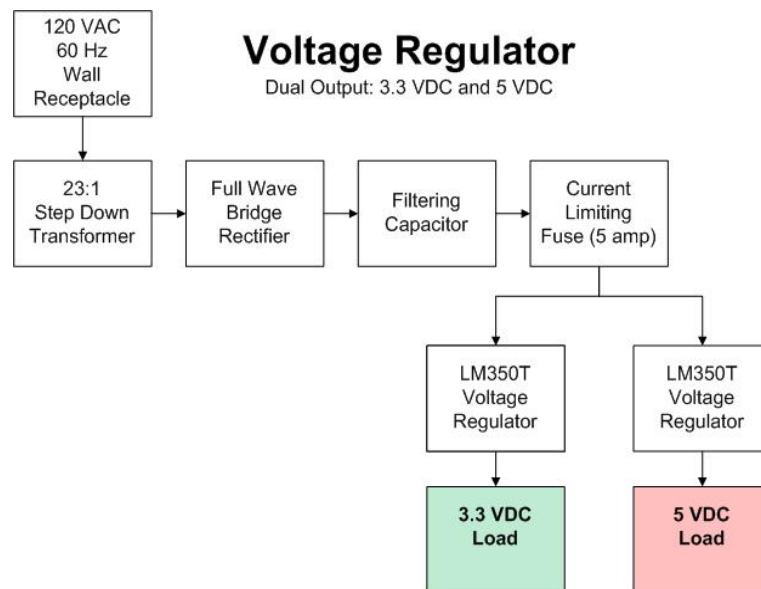
Figure 3.4a- Dual Voltage Regulator
