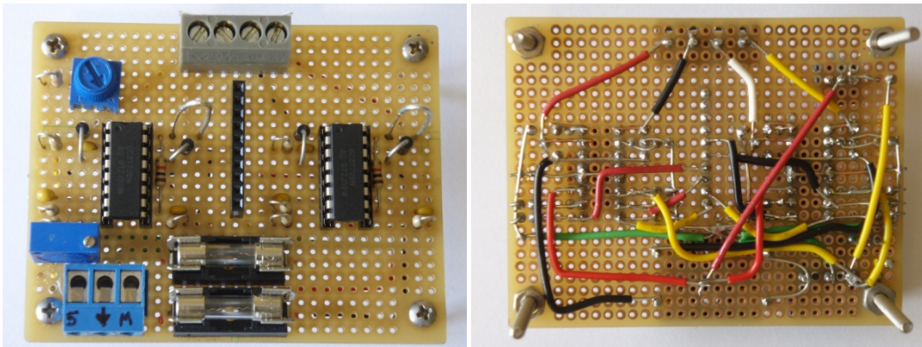
Figure 3.3d- Top and Bottom View of the Motor Driver Circuit
