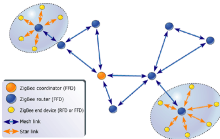
Figure 2.9.3a- Combined Integration of Star and Mesh topologies
