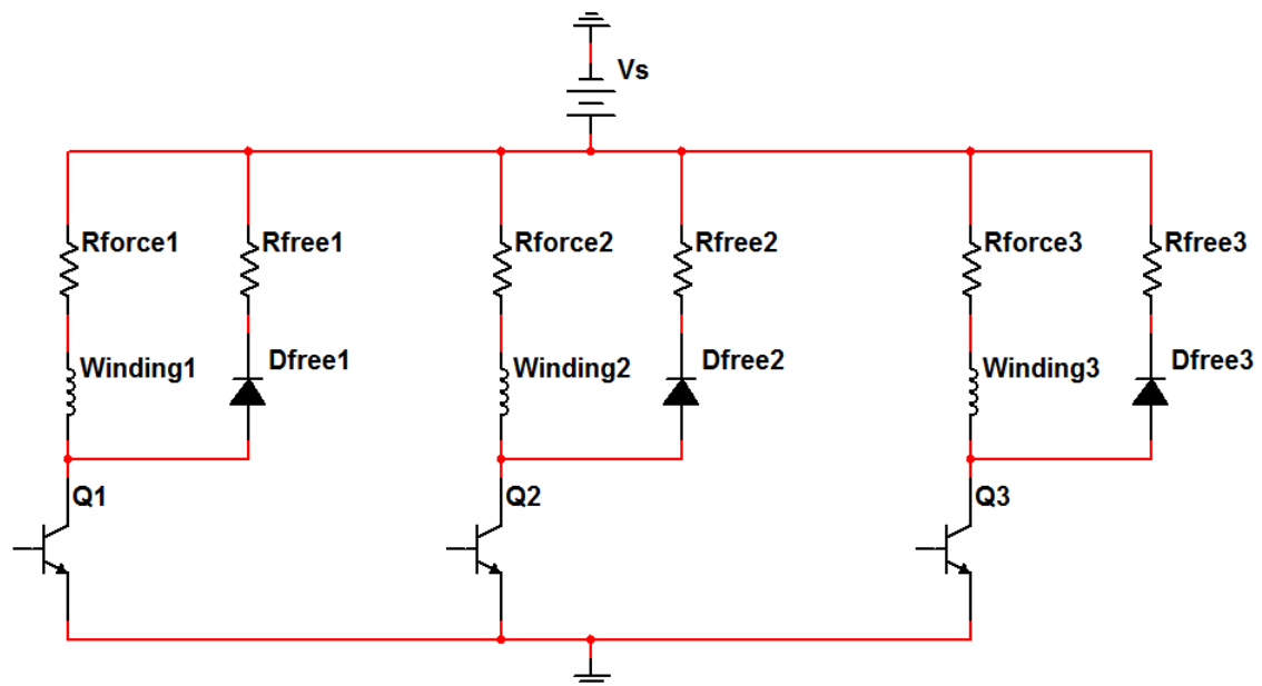
Figure 2.2.1a: Depiction of a Unipolar Driver Circuit
