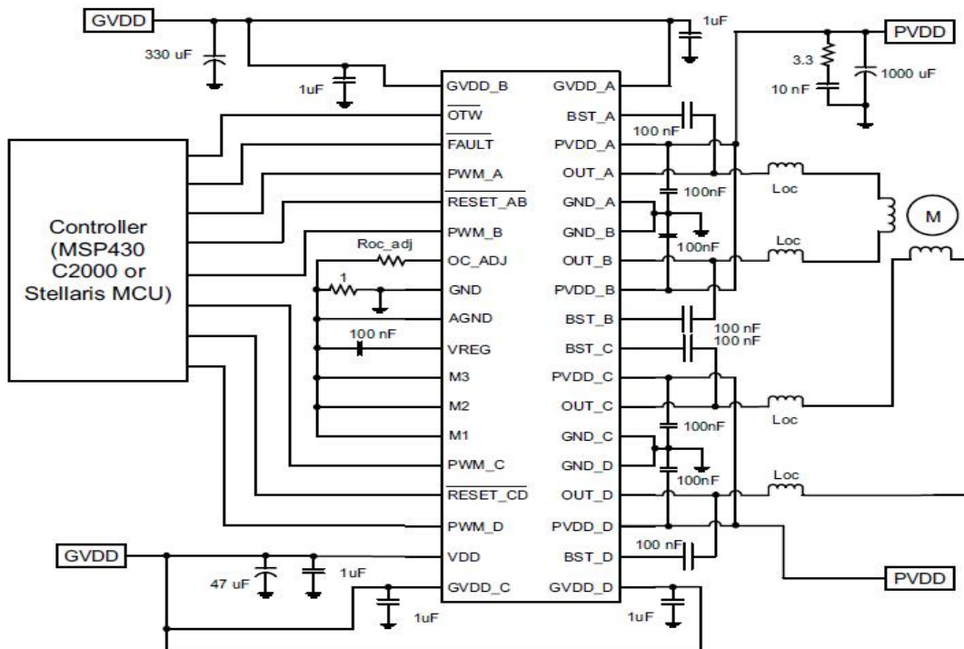
Circuit Schematic 4.2a – Motor driver Schematic [A1]
