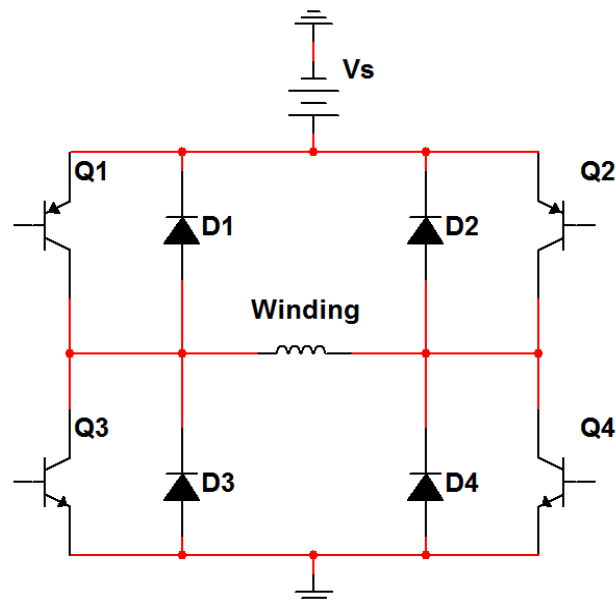
Figure 2.2.2a: Depiction of a Bipolar H-Bridge Driver Circuit
