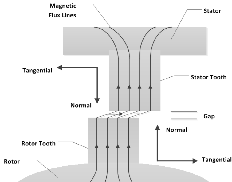
Figure 2.1a: Depiction of the magnetic forces upon the stepper motor teeth
