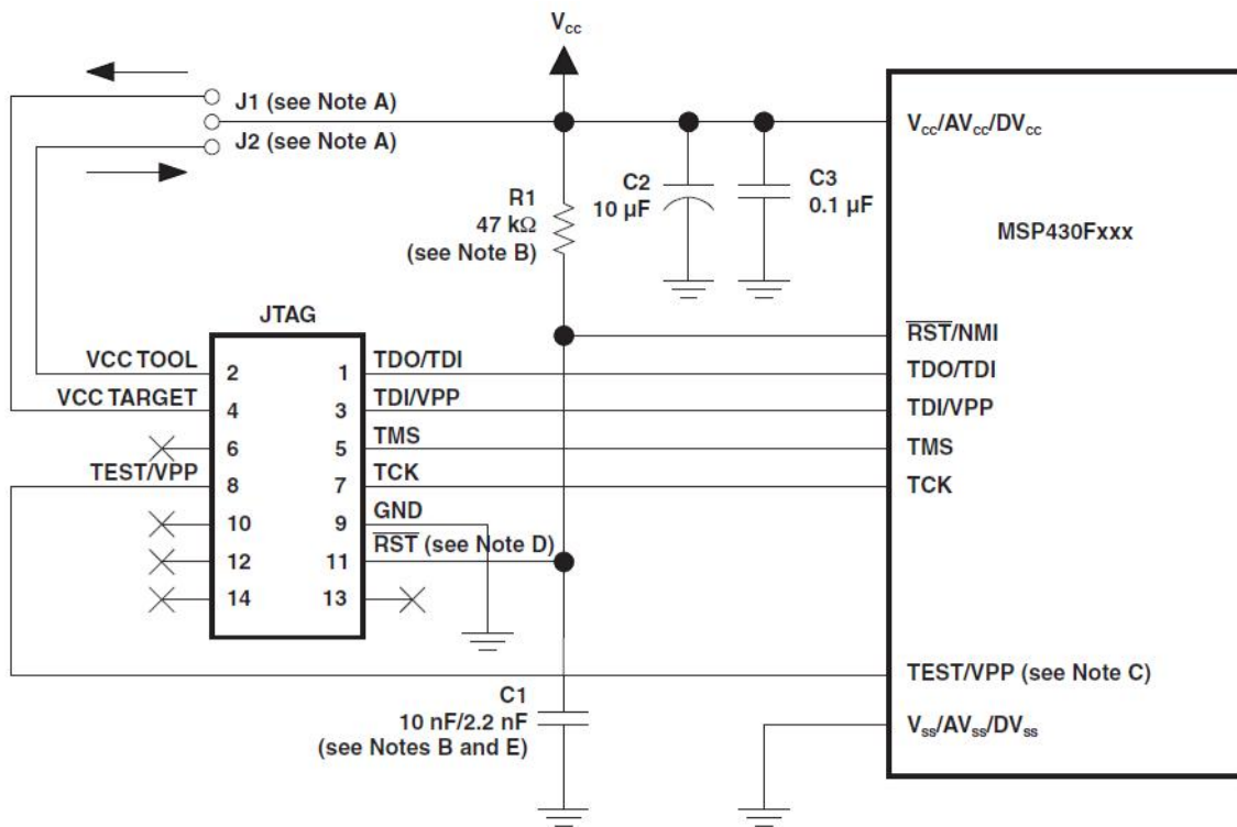
Figure 4.6.8a- Recommended JTAG connection. [A4]
