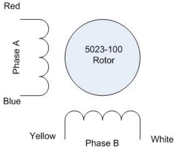
Figure 3.2b- Stepper Motor Winding Configuration
