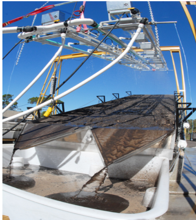
Figure 1.1a- Rain Simulator at UCF [B1]
