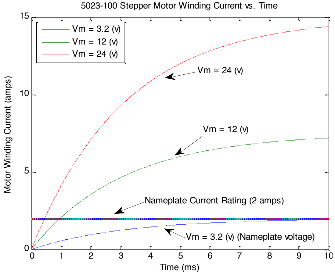
Figure 3.3b- Step Response
