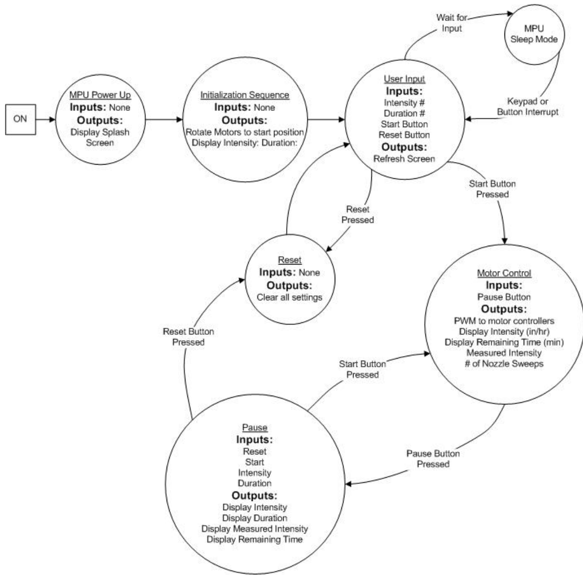
Figure 4.6.1a- Rain Simulator Software State Machine
