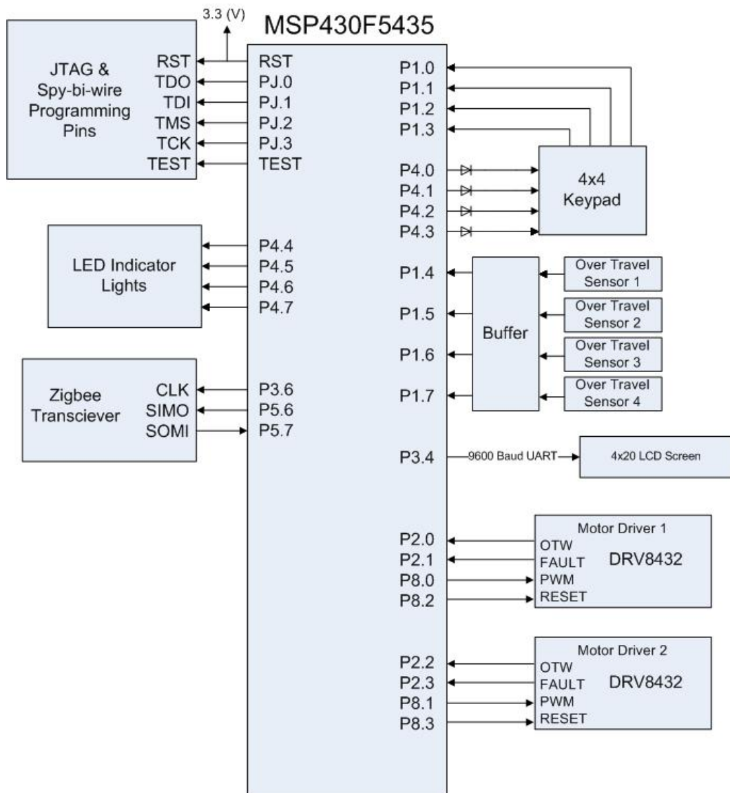
Figure 4.6.3a- Port and Pin Assignments for the Final Project
