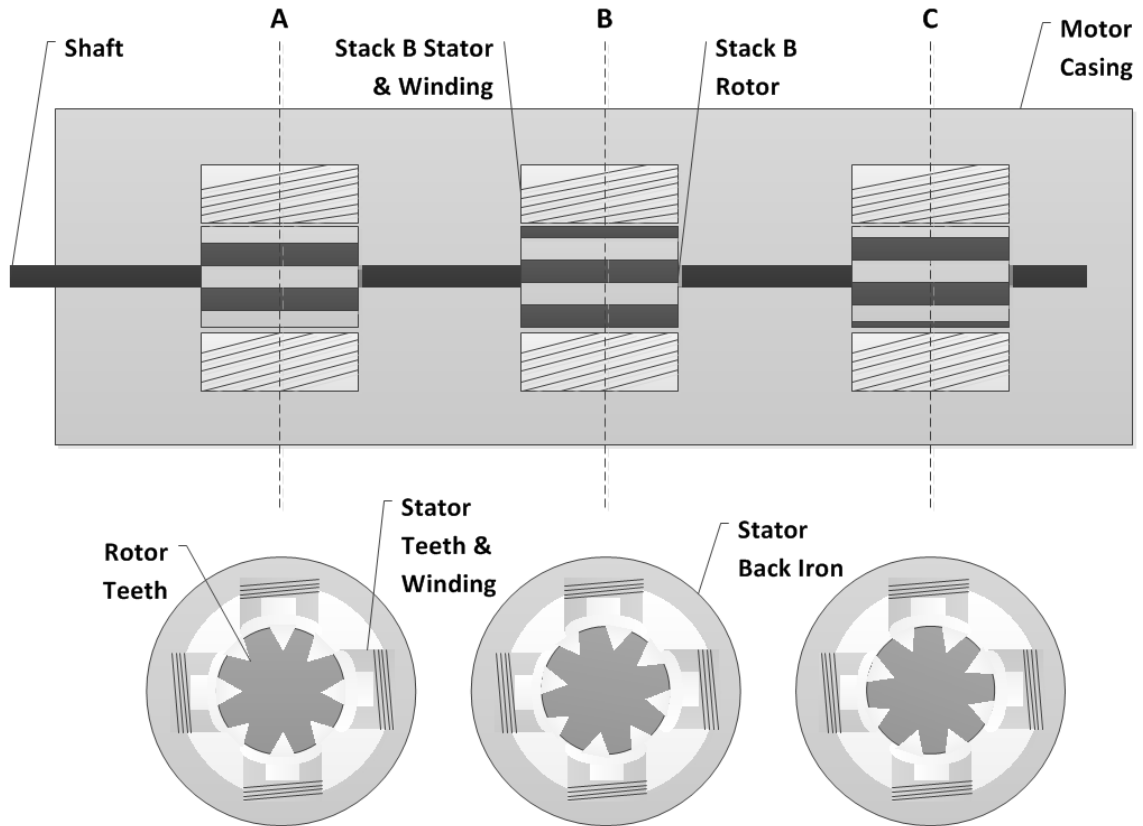
Figure 2.1.2a: Depiction of the Variable Reluctance Stepper Motor Construction
