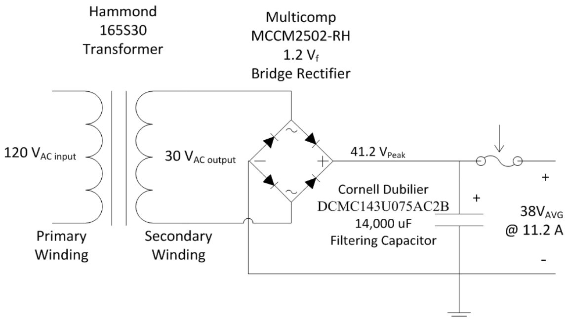
Figure 4.3.4a: Schematic of Design Summary for High Voltage Power Supply
