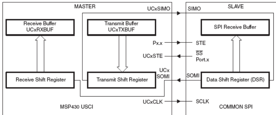
Figure 2.5.2a- SPI Interface Master Mode [L8] Connections from Master to Slave in 3 or 4 wire mode. (Permission Granted by Texas Instruments)
