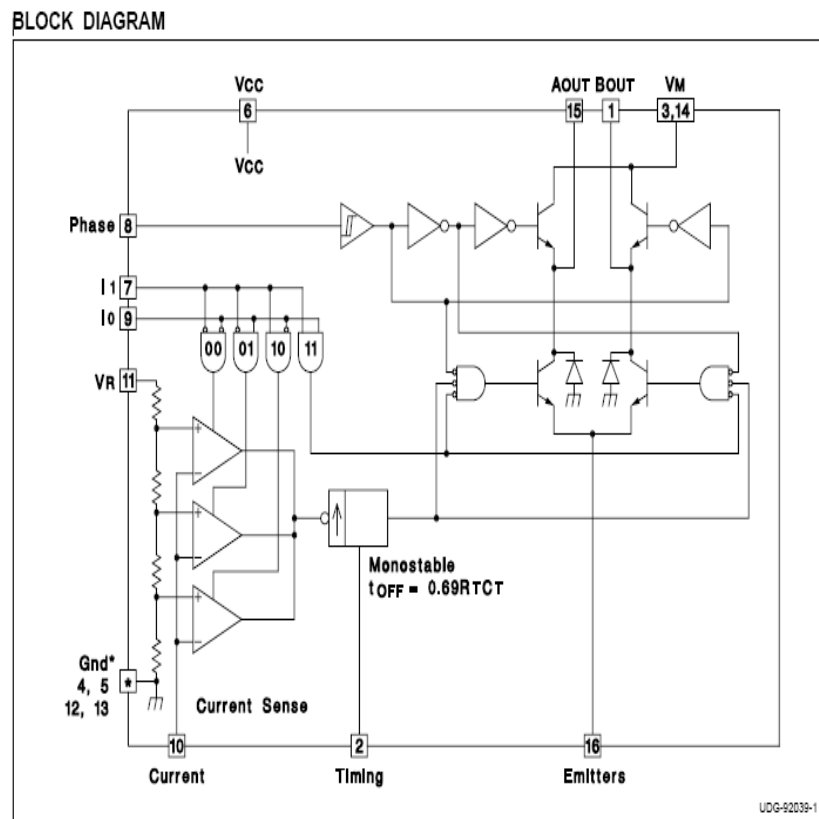
Figure 3.3a- UC3770BN Block Diagram [L6]
